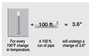
Rule of Thumb for PVC Expansion
